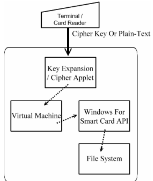
Figure 6: Internal COS Process of Key Expansion and Cipher Applets
