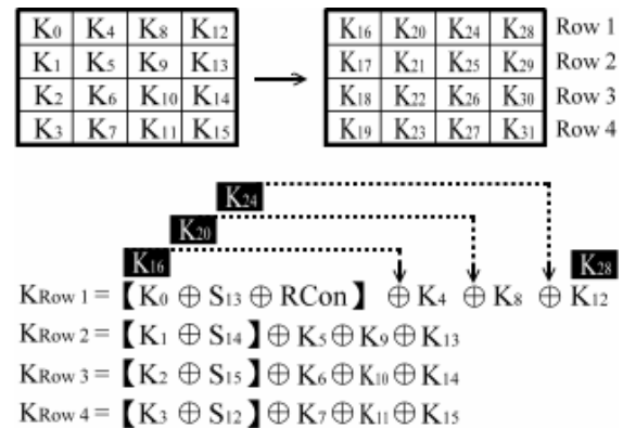
Figure 5: Suggested Round Key Process
