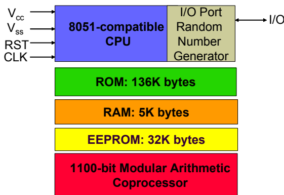
Figure 2: Block diagram of SLE66CX322P
