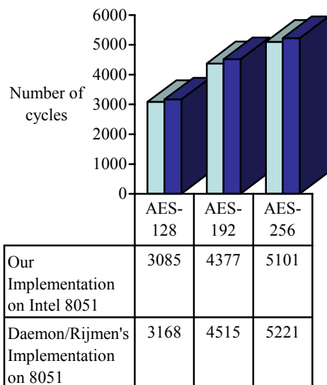
Figure 7: The Comparison of Daemon/Rijmen [5] and Our Implementation Results
